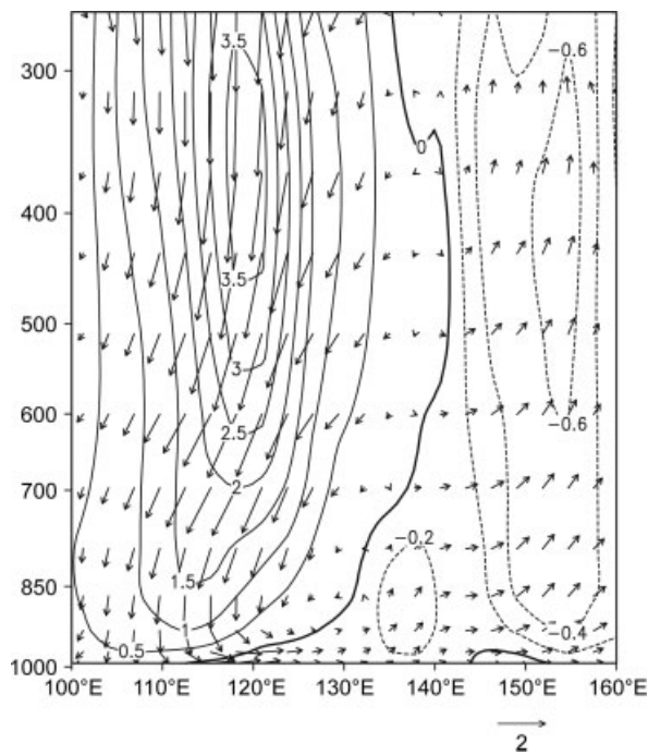
Figure 8. The zonal-height distribution of differences between sensitivity experiment with cooling SST over Wharton Basin and control run.
