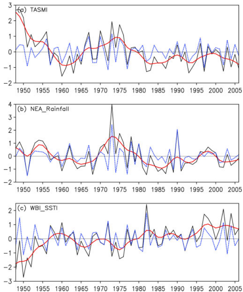
Figure 2. (a) Normalized time series of TSMI (solid line). The thick solid (dashed) lines indicate the interdecadal (interannual) variation filtered by a 7-year Gaussian filter. (b) As for (a), but for the NEA summer rainfall series. (c) As for (a), but for WB-SSTI, which is the areal-averaged SST over the Wharton Basin ( 100^{\circ} – 130^{\circ} E, 20^{\circ} – 5^{\circ} S). This figure is available in colour online at wileyonlinelibrary.com/journal/joc
