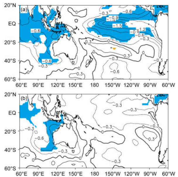
Figure 6. (a) Composite difference in SST between strong and weak TASM years. (b) As for (a), but for non-ENS0 years. Shading indicates statistically significant difference at the 0.01 level. This figure is available in colour online at wileyonlinelibrary.com/journal/joc
