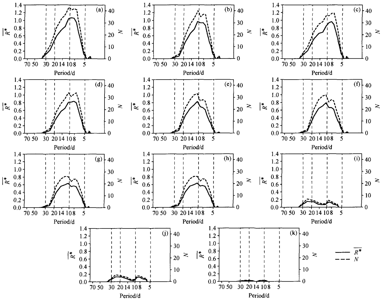
图7 同图5, 但为NAMI非活跃期(5~9月) Fig. 7 Same as Fig. 5, except for NAMI in the non-active period (from May to Sep)
